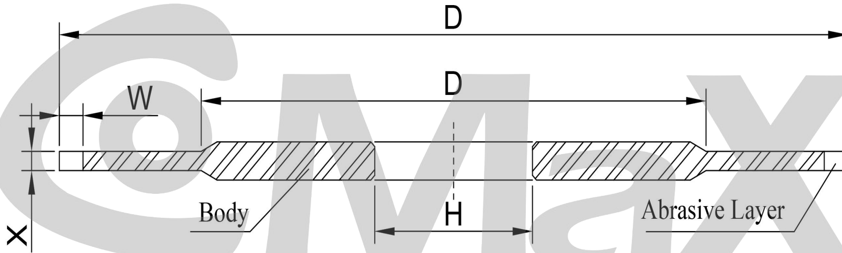
SECTION VIEW
